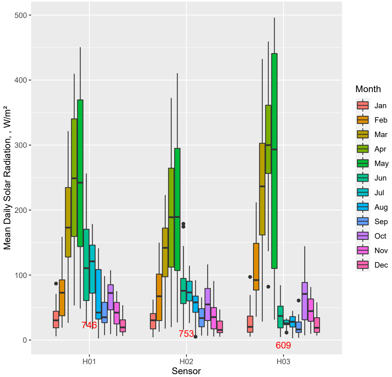
Mean Daily Solar Radiation per Sensor per Month
